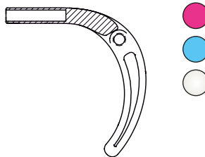
7.2 SFLOb endpiece raster hook gap
